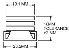
MIN/MAX WORKING CLEARANCE
