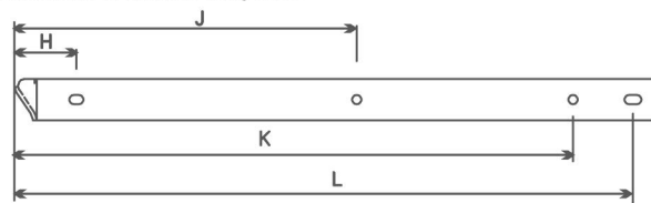
Underside of channel fixing holes
